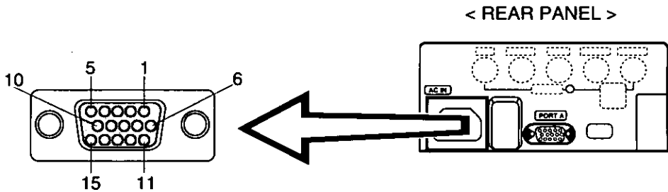
Pin assignments of 15-pin mini D-Sub connector
